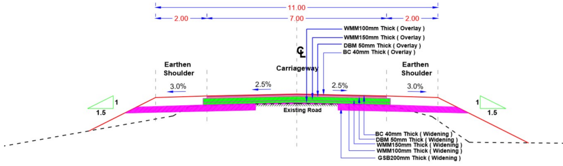
TYPICAL CROSS SECTIONS – IV
