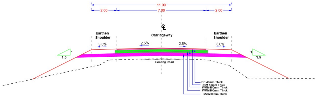
TYPICAL CROSS SECTIONS – V
